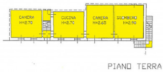
PIANO TERRA
